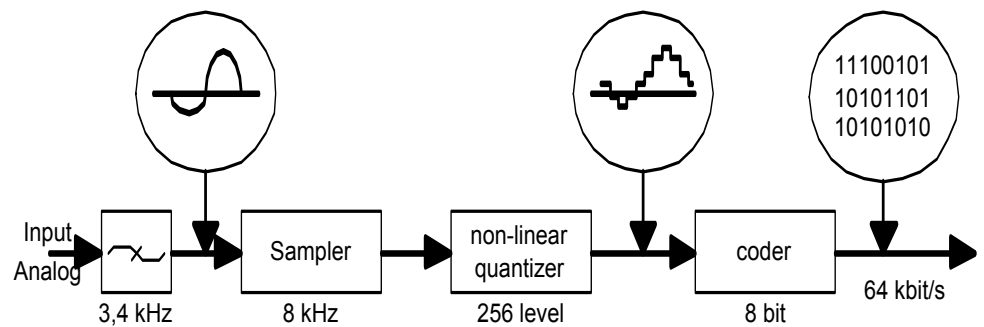
Gambar 1 Pengkodean Pulse Code Modulation
